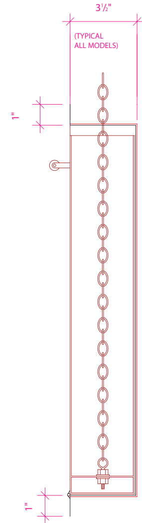
SECTION THRU HOUSING SIDE
