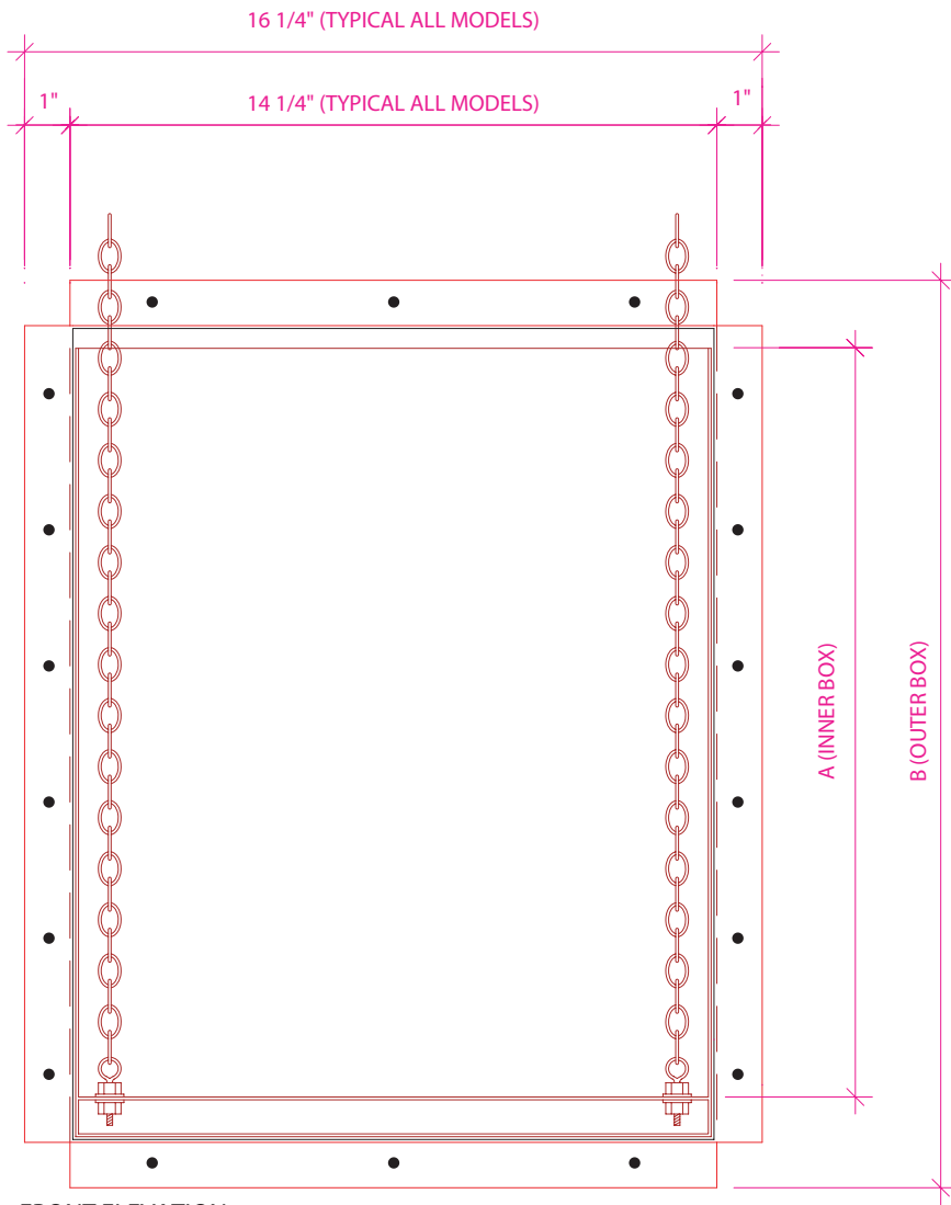
FRONT ELEVATION
